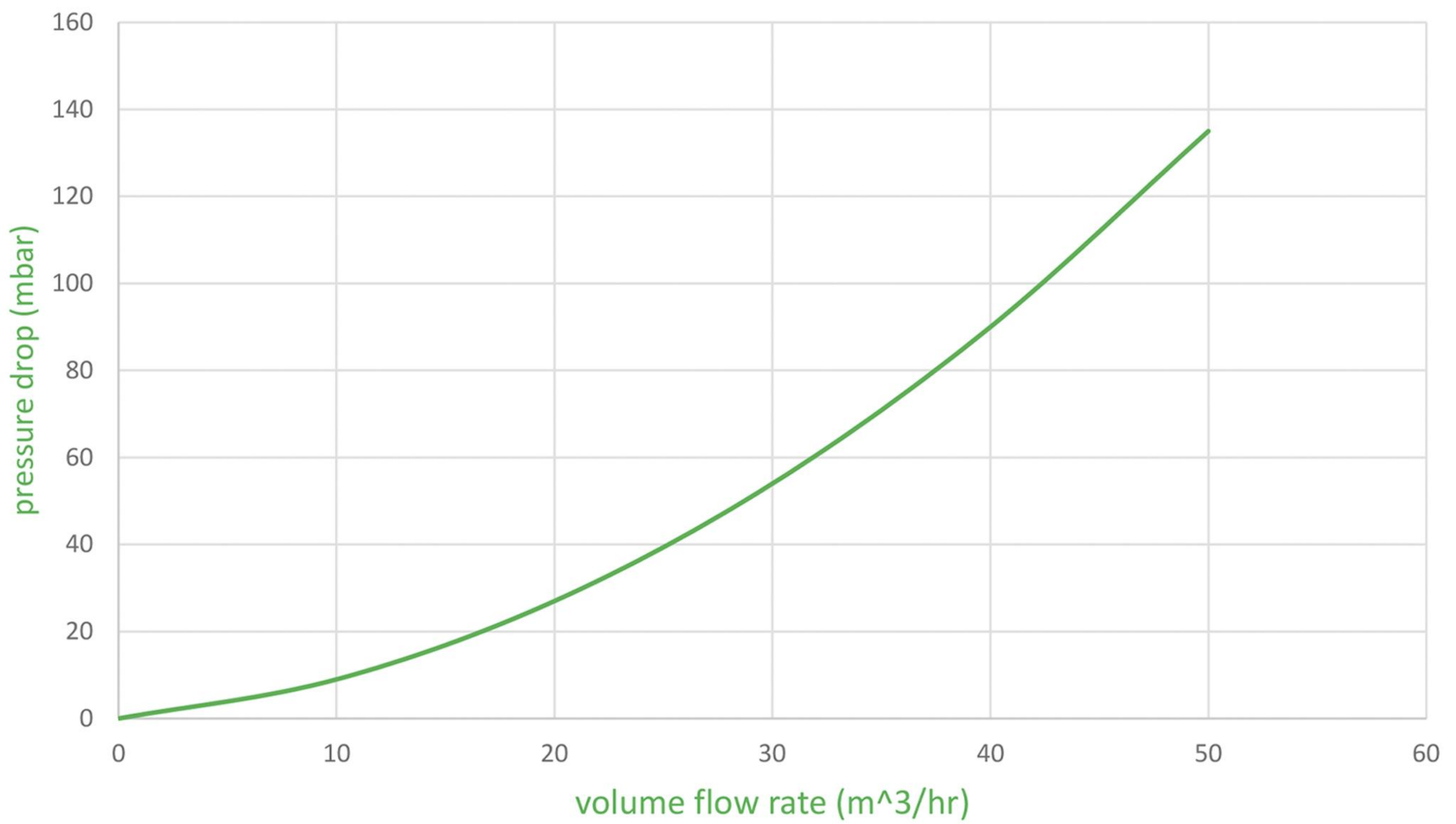
SS.T pressure drop vs flow curve
